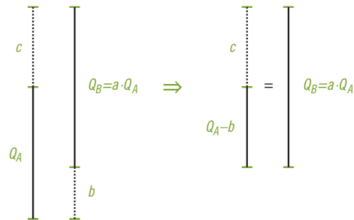
Figure 1: A hypothetical quantitative structure.
